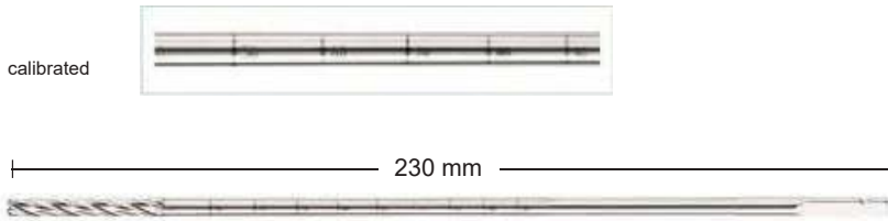
Drill for three-jaw chuck, cannulated four-edged
